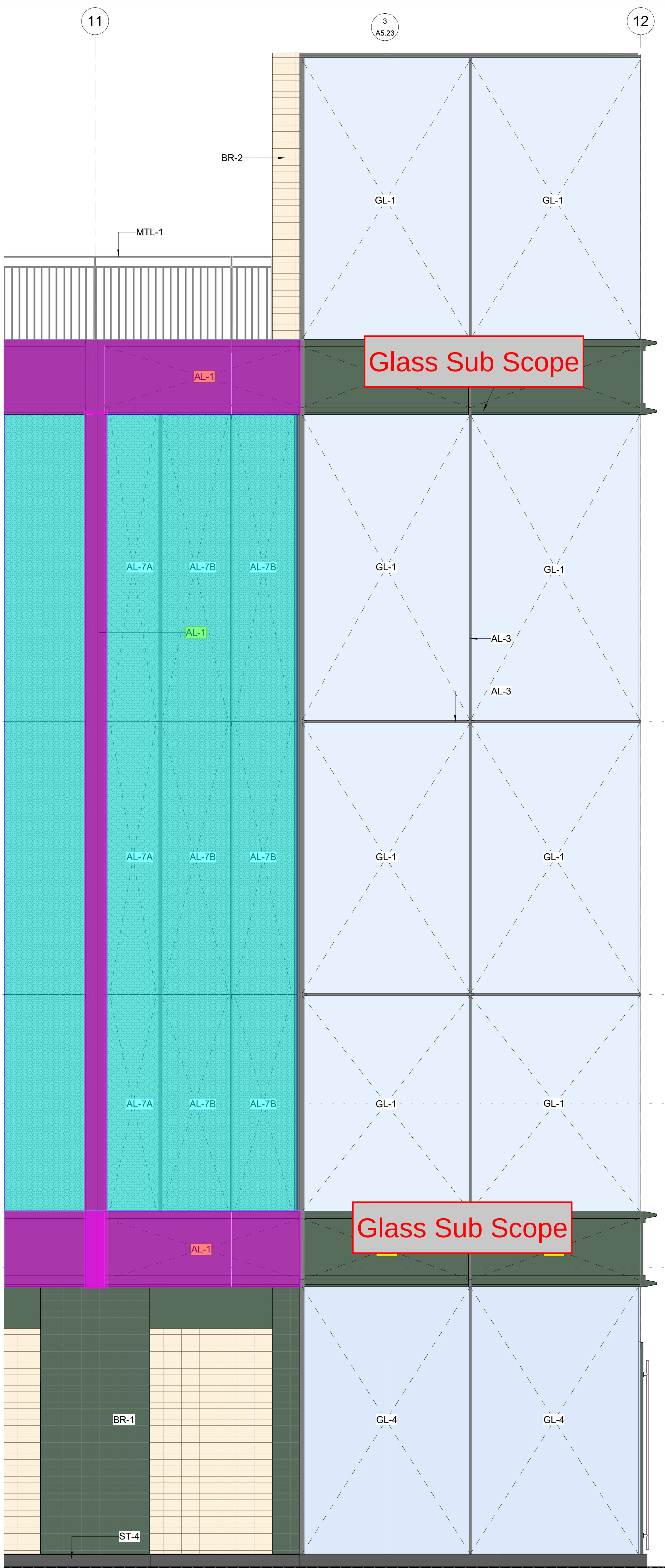
1 ENCLOSURE TYPE B1 - GARAGE SOUTH - ELEVATION 1/2" = 1'-0"
