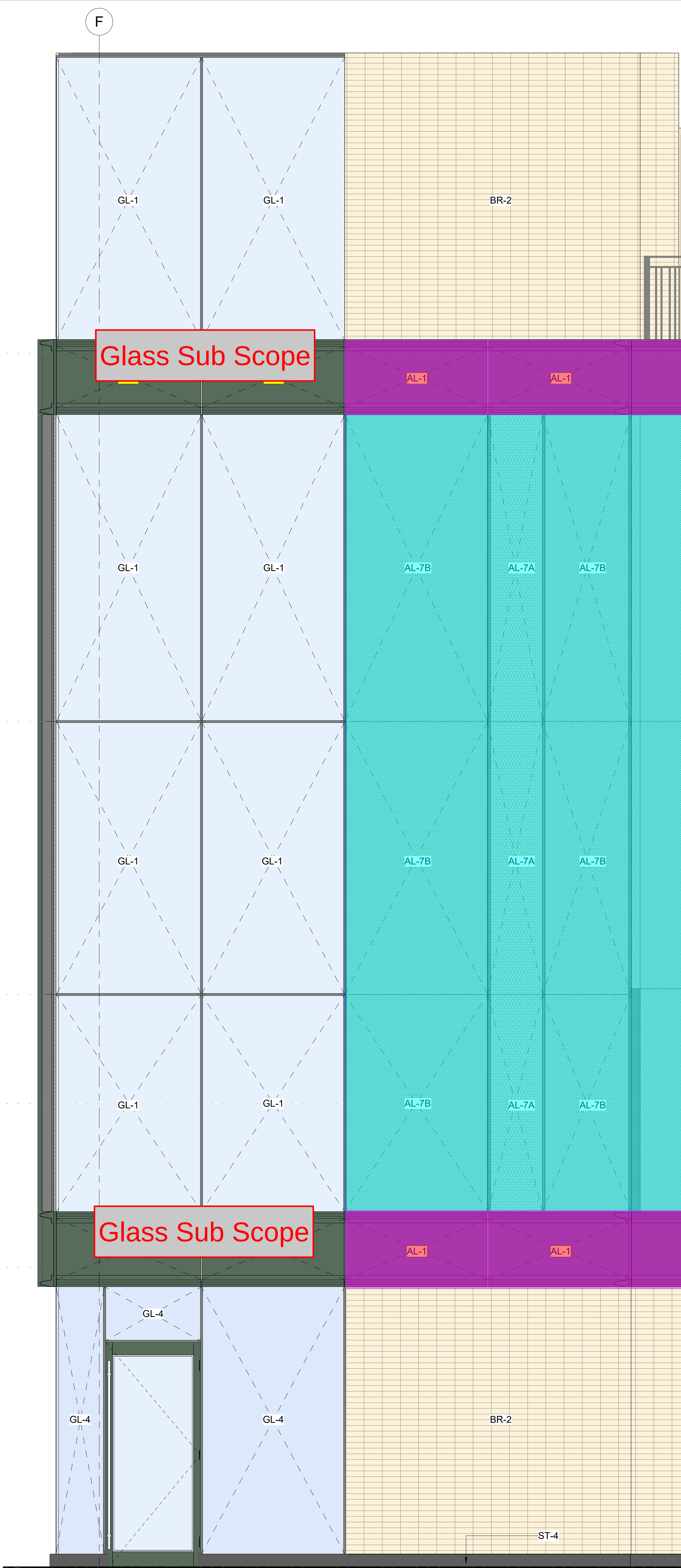
2 ENCLOSURE TYPE B1 - GARAGE SOUTH ELEVATION 2 1/2" = 1'-0"
